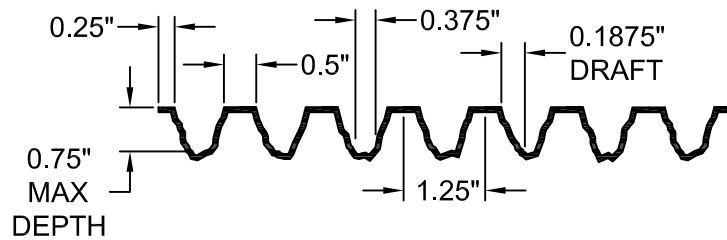
FORMLINER DETAIL
