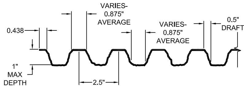
FORMLINER DETAIL
