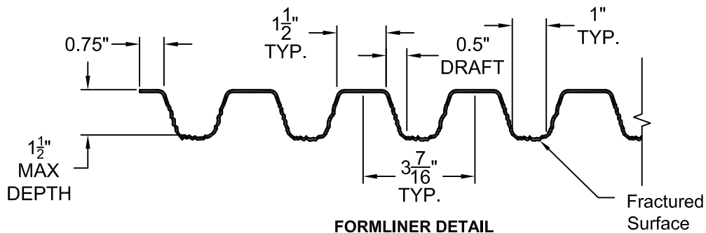
FORMLINER DETAIL
