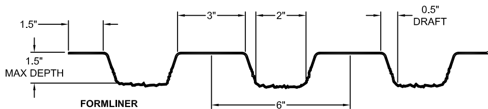
FORMLINER DETAIL
