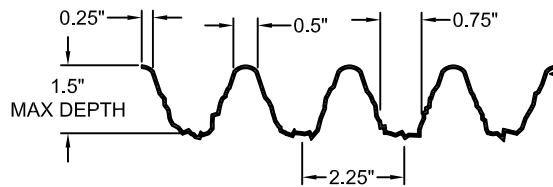
FORMLINER DETAIL
