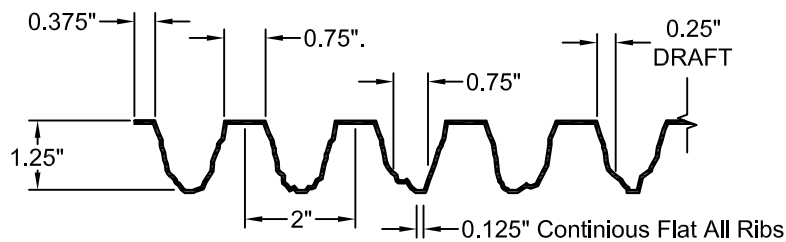
FORMLINER DETAIL
