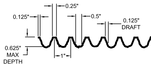
FORMLINER DETAIL
