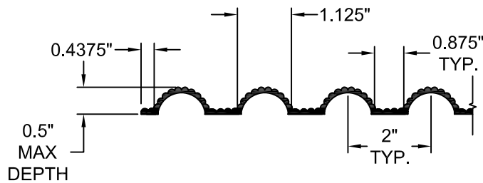
FORMLINER DETAIL
