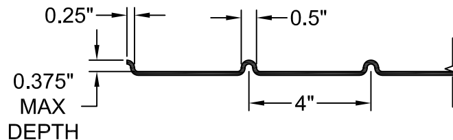
FORMLINER DETAIL
