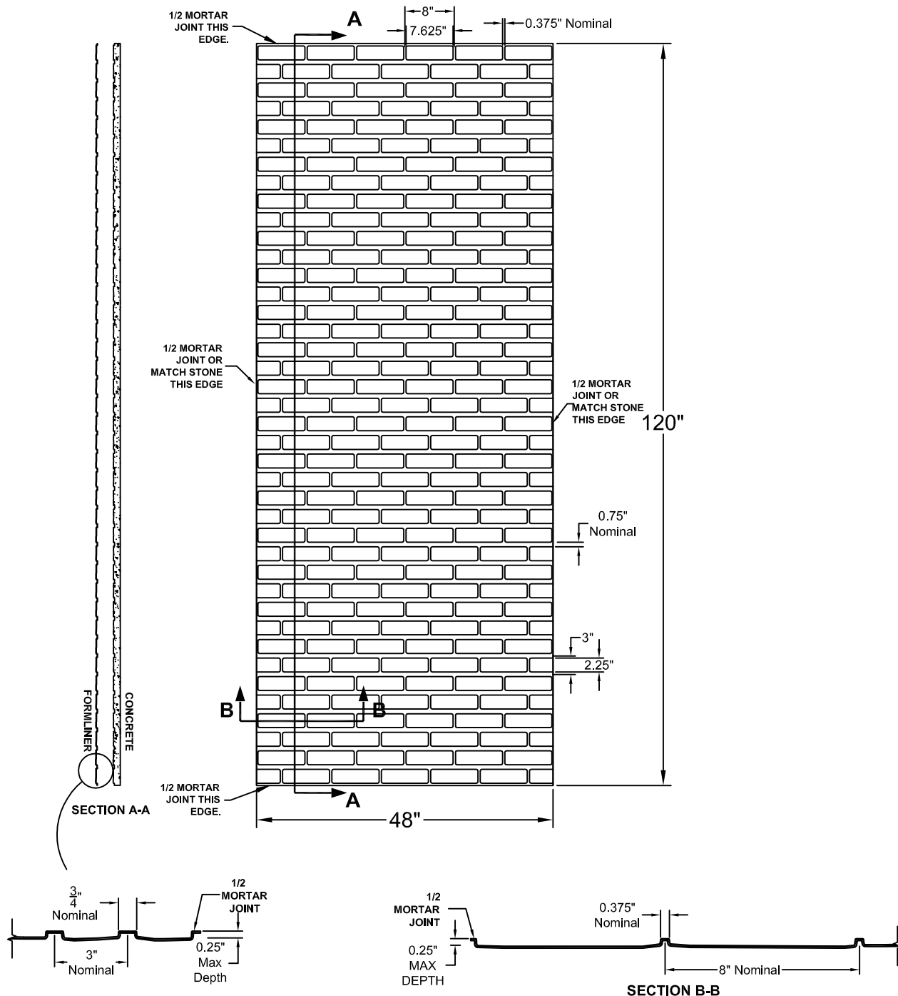
FORMLINER DETAIL
