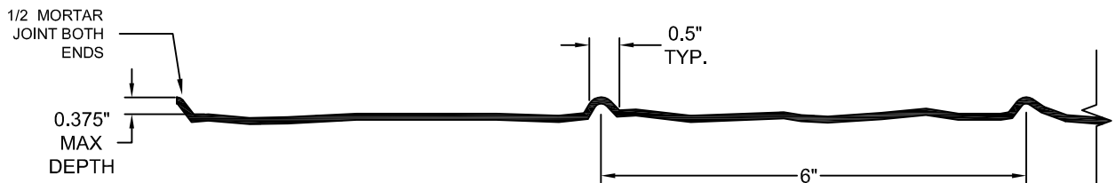
FORMLINER DETAIL
