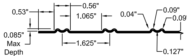
FORMLINER DETAIL
