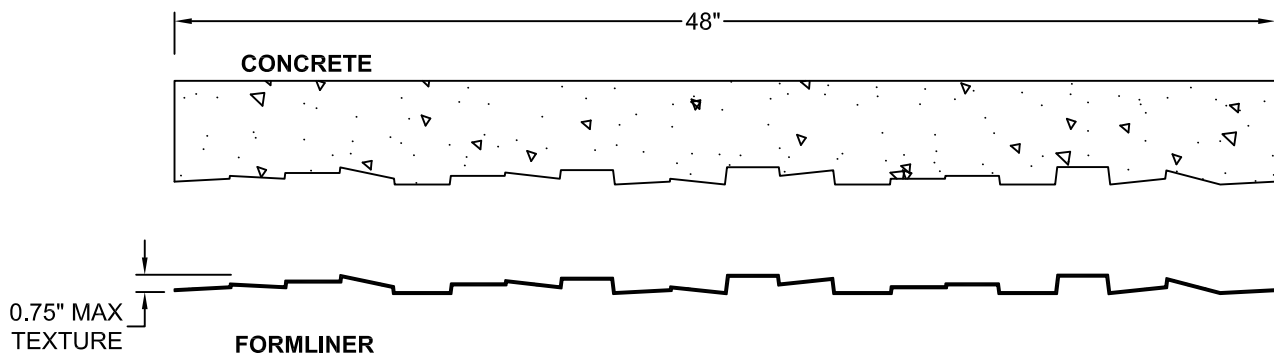
SECTION A-A FORMLINER DETAIL
