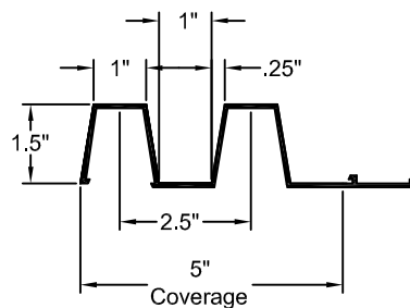
FORMLINER DETAIL
