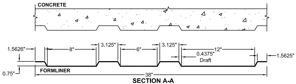
SECTION A-A FORMLINER DETAIL
