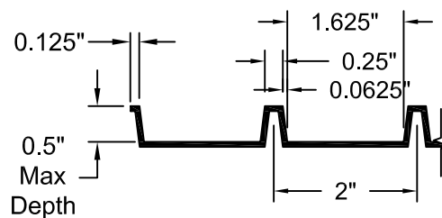
FORMLINER DETAIL
