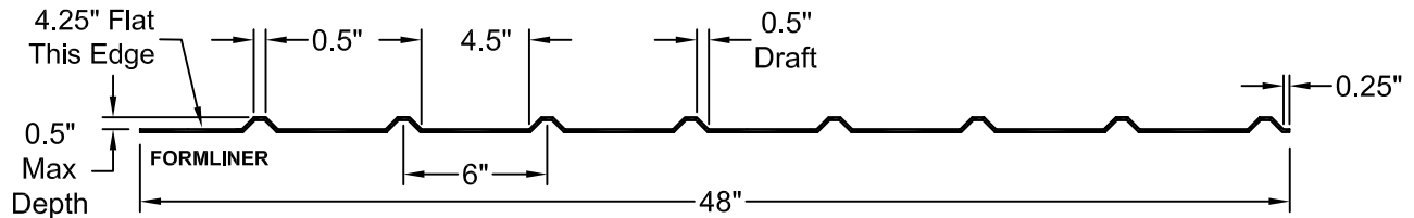
SECTION A-A FORMLINER DETAIL
