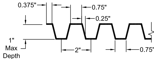
FORMLINER DETAIL
