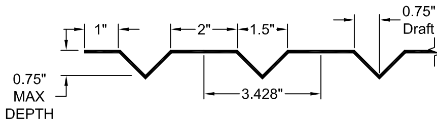
FORMLINER DETAIL
