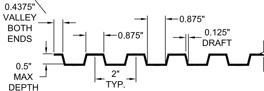
FORMLINER DETAIL
