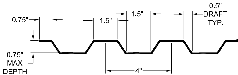
FORMLINER DETAIL
