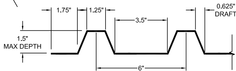
FORMLINER DETAIL
