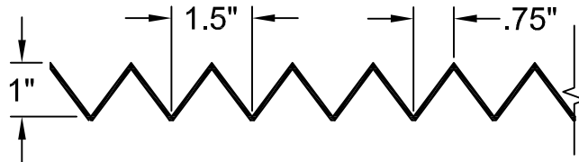
FORMLINER DETAIL
