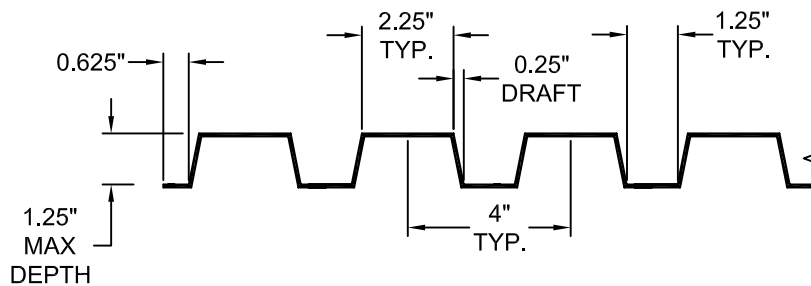
FORMLINER DETAIL
