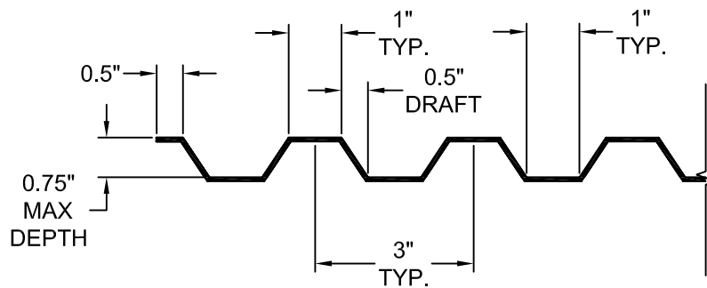
FORMLINER DETAIL
