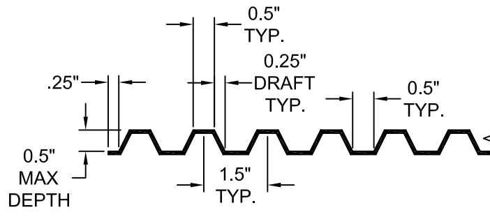
FORMLINER DETAIL
