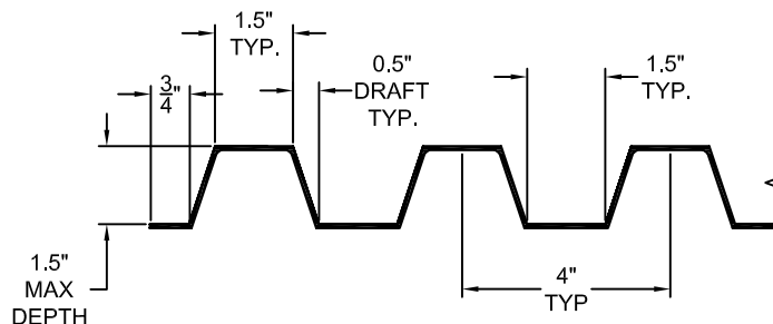
FORMLINER DETAIL
