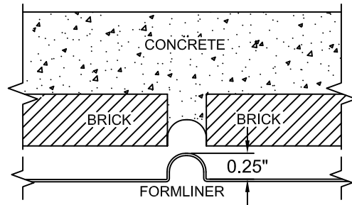
FORMLINER DETAIL
