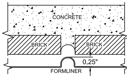
FORMLINER DETAIL
