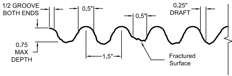
FORMLINER DETAIL
