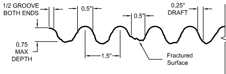
FORMLINER DETAIL
