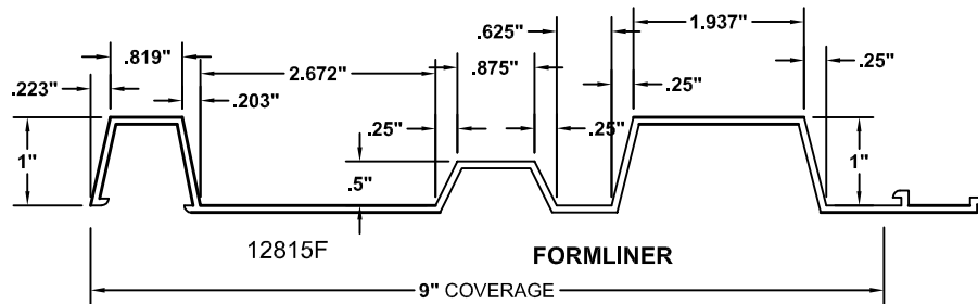
FORMLINER DETAIL
