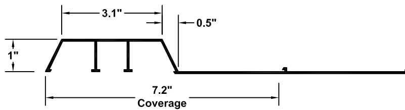
FORMLINER DETAIL
