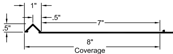
FORMLINER DETAIL
