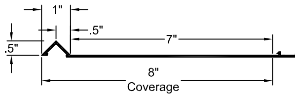
FORMLINER DETAIL
