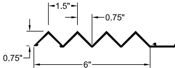
FORMLINER DETAIL
