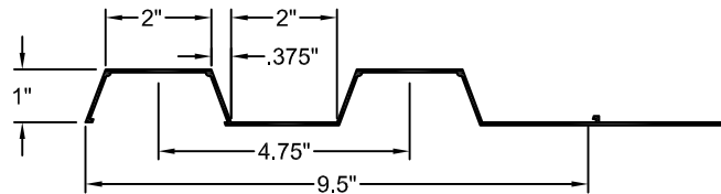
FORMLINER DETAIL
