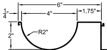
FORMLINER DETAIL
