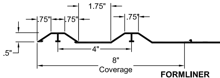
FORMLINER DETAIL
