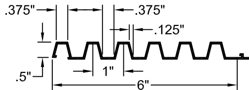
FORMLINER DETAIL
