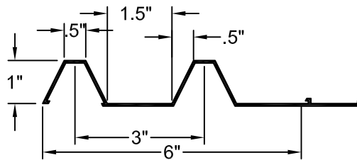
FORMLINER DETAIL
