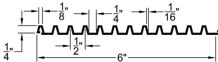
FORMLINER DETAIL
