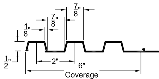
FORMLINER DETAIL
