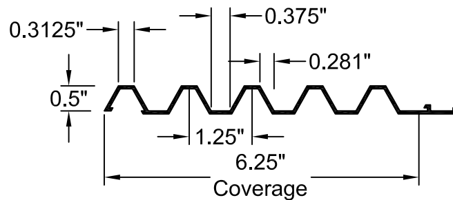
FORMLINER DETAIL
