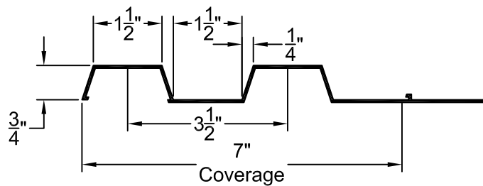
FORMLINER DETAIL
