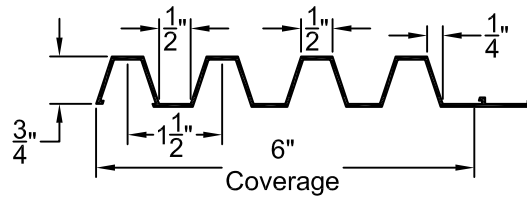
FORMLINER DETAIL
