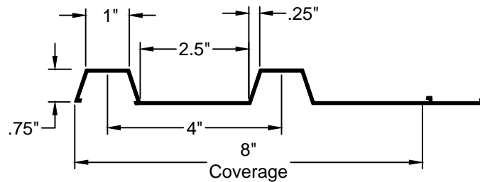
FORMLINER DETAIL
