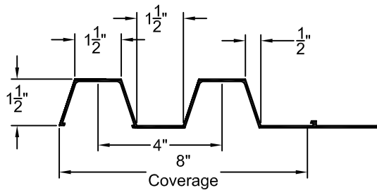
FORMLINER DETAIL
