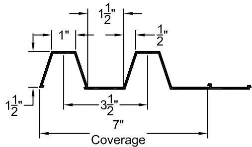
FORMLINER DETAIL
