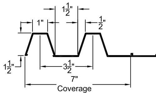
FORMLINER DETAIL
