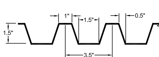
FORMLINER DETAIL
