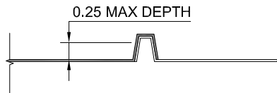
FORMLINER DETAIL
