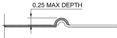
FORMLINER DETAIL
